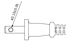
Non-Polarized
